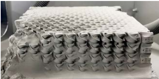
Depowdering full print box of Digital Metal logos
